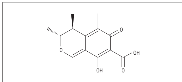
Figure 2. Chemical structure of citrinin. H indicates hydrogen; O, oxygen.
