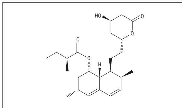
Figure 1. Chemical structure of monacolin K (lovastatin). H indicates hydrogen; O, oxygen.
